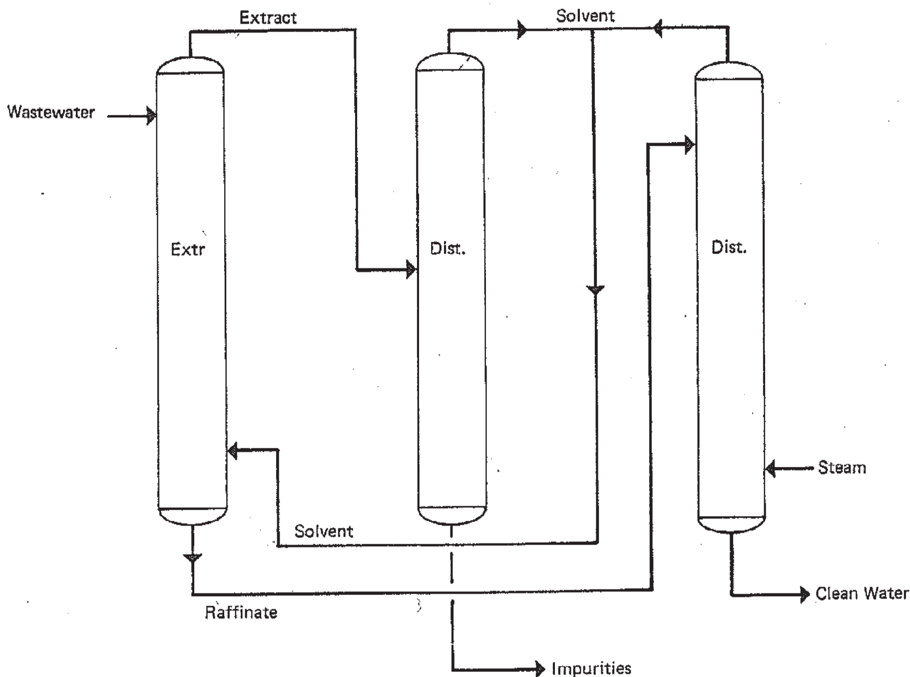
Figure 1. Solvent extraction process.
